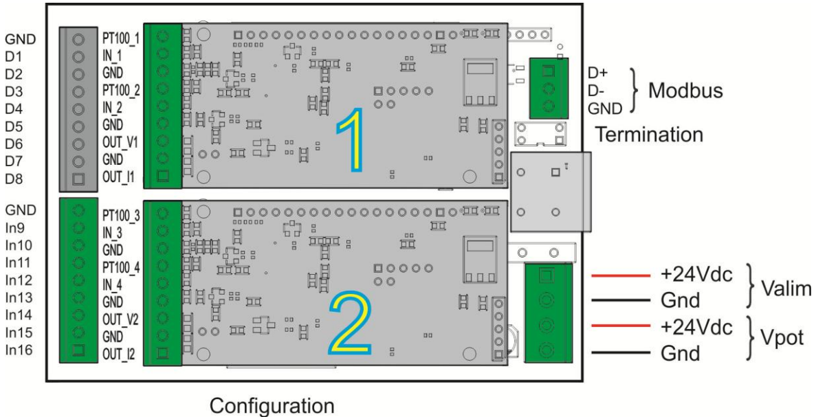
Fig.: Connection of the base + analog inputs / output (Expansion boards)
