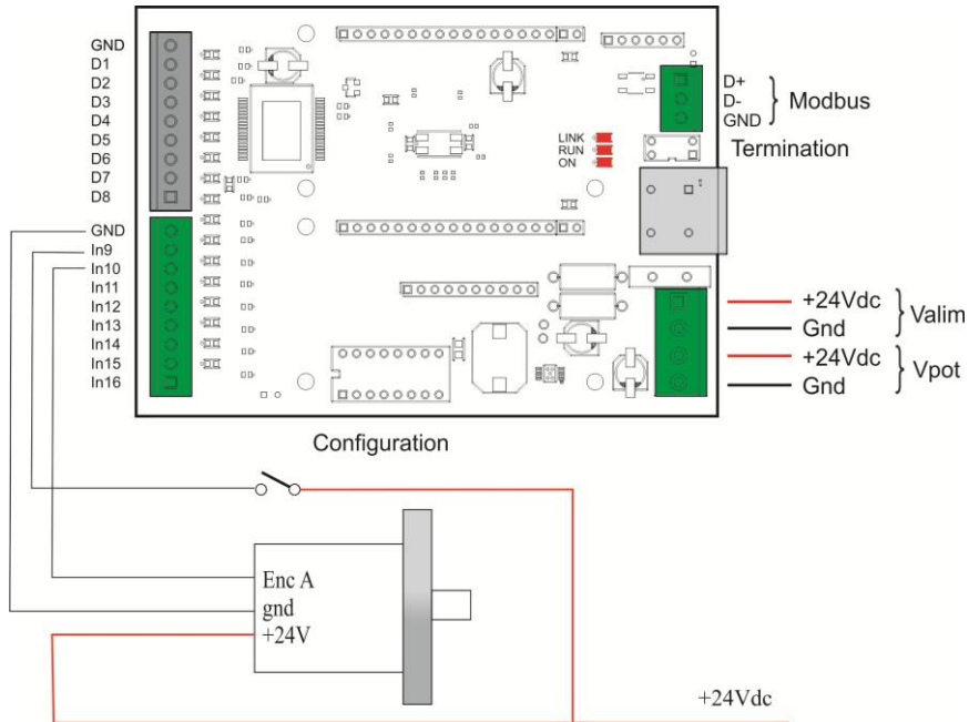
Fig.: Unidirectional encoder connection
